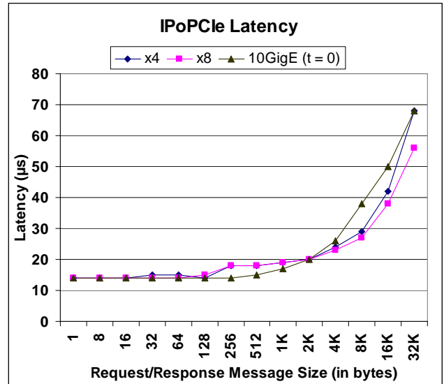
Figure 7 Comparing the IPoPCIE latencies with that of the best latencies obtained on a 10GigE setup (wherein interrupt coalescing is completely disabled)
