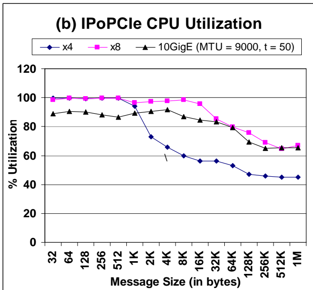
Figure 8 Comparing the IPoPCIe bandwidth and receive side CPU utilization with that of the best bandwidth/CPU utilization obtained on a 10GigE setup (interrupt coalescing timer set at 50μs and jumbo frames used)
