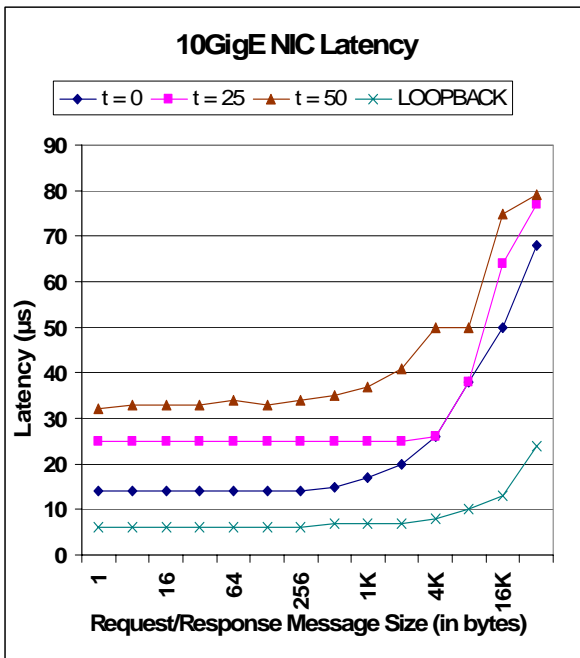
Figure 5 Illustration shows the latency for varying message sizes as well as the effect of changing the interrupt coalescing timer. A timer value of 0 ( t = 0 ) indicates that interrupt coalescing is disabled.
